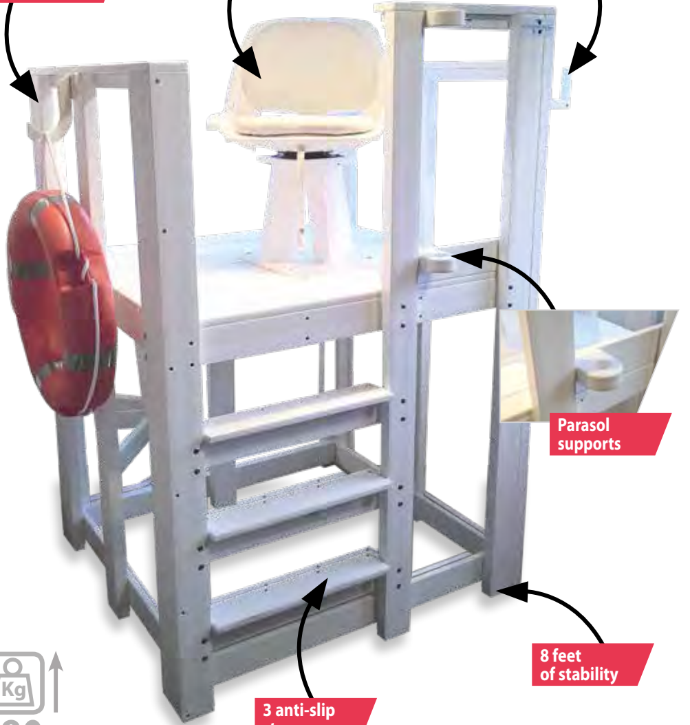
Buoy holder hook
