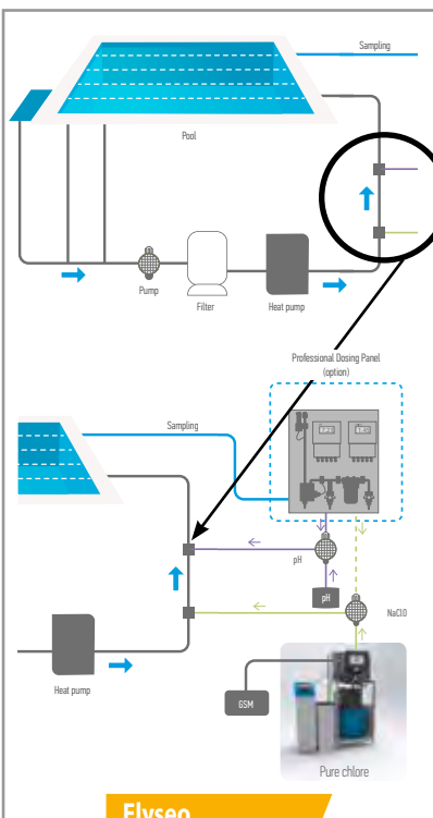
Elyseo installation diagram
